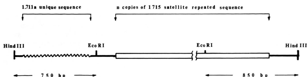
Fig. 4. The schematic presentation of the family of Hind III fragments containing “ n ” copies of the 1.715 satellite repeated sequence, flanked with not related sequence regionally homologous to 1.711a satellite unique sequence.
